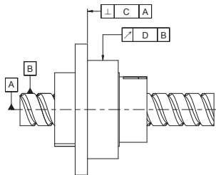
Fig 1.2.3 RFBY - series
