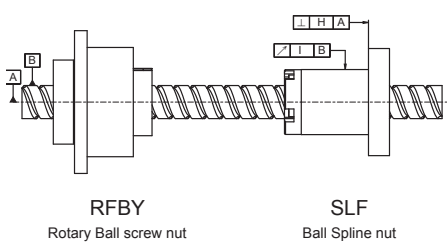
Fig 1.2.2 RBLY - series
