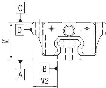
Fig 2.2.5 Accuracy Standard
