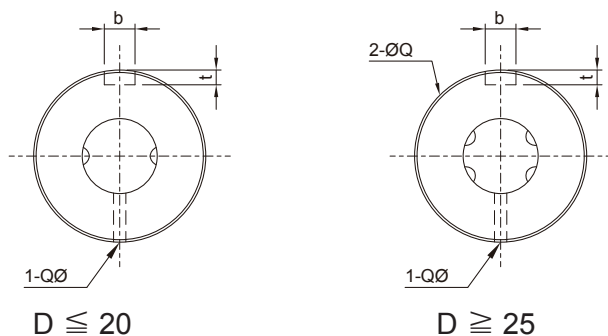
Hollow Spline Shaft
